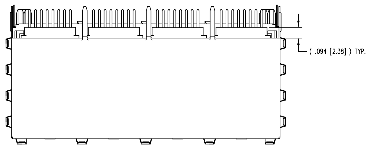
PIN DETAIL TYP. ALL PORTS
