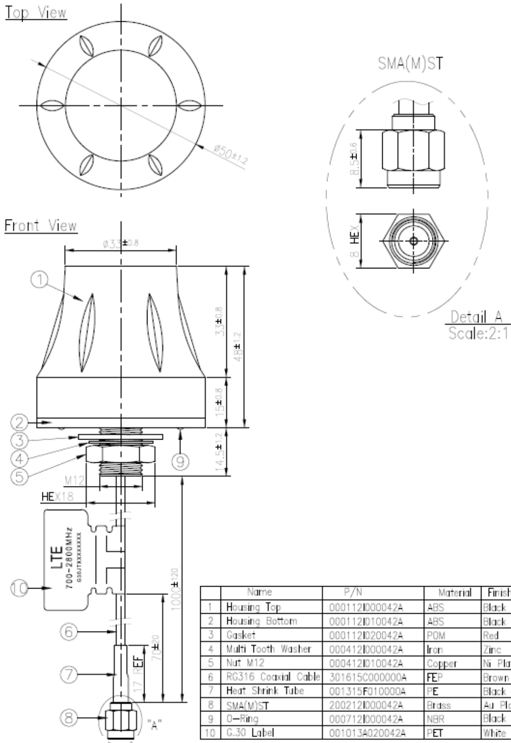
Figure 37. Mechanical Drawing of the G30 Antenna
