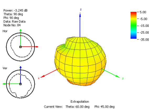
Figure 22. Radiation Pattern at 1805MHz of G30 Antenna in Free Space
