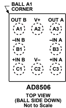
Figure 4. 8-Ball WLCSP (CB-8-2)
