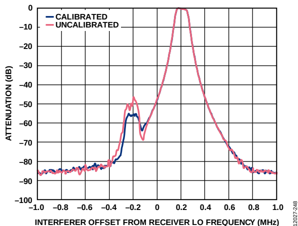
Figure 31. Image Attenuation with Calibrated and Uncalibrated Images, 433 MHz, IF Filter Bandwidth = 100 kHz, V_{DD} = 3.0 V, Temperature = 25°C
