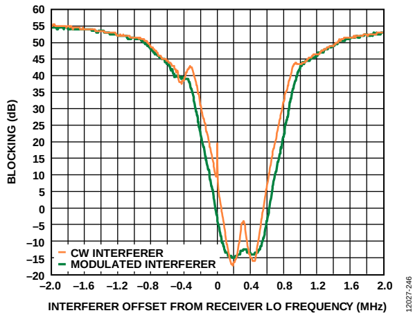
Figure 29. Receiver Close-In Blocking at 915 MHz, Radio Profile F, Image Calibrated
