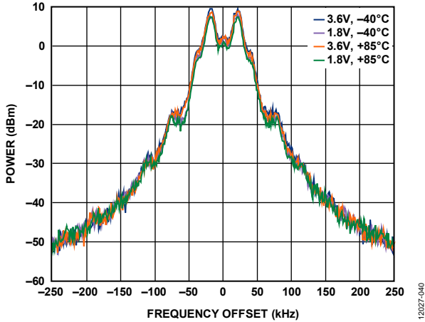
Figure 11. Transmit Spectrum at 868 MHz, FSK, Radio Profile B, (Minimum Recommended V_{DD} = 2.2\text{ V} , 1.8 V Operation Shown for Robustness)
