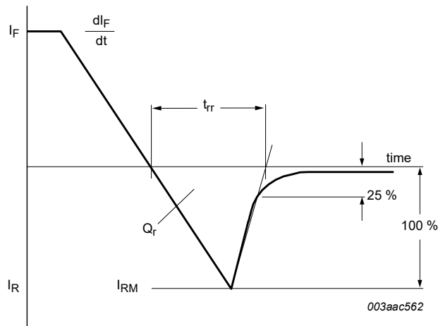
Fig. 9. Reverse recovery definitions; ramp recovery
