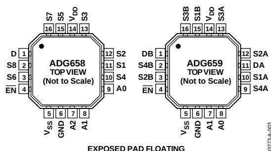
Figure 3. 16-Lead, 4 mm x 4 mm LFCSP Pin Configuration
