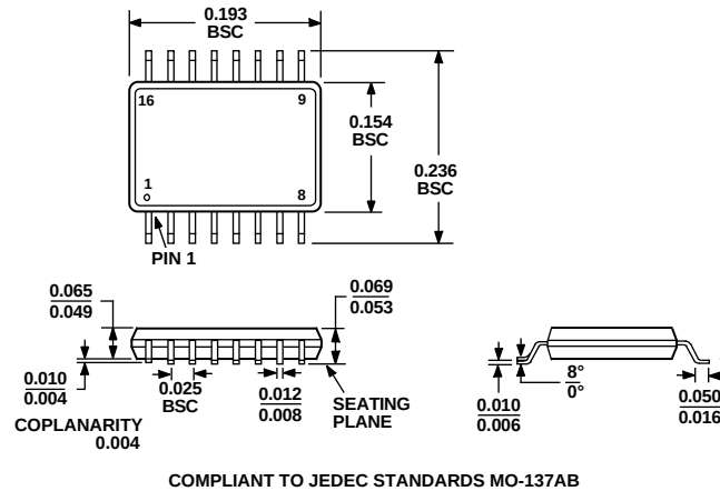
Figure 34. 16-Lead Shrink Small Outline Package [QSOP] (RQ-16) Dimensions shown in millimeters
