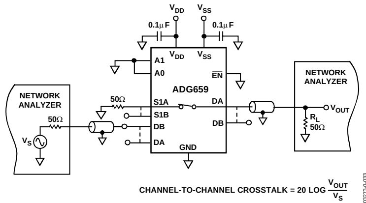
Figure 31. Channel-to-Channel Crosstalk
