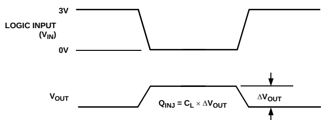
Figure 28. Charge Injection
