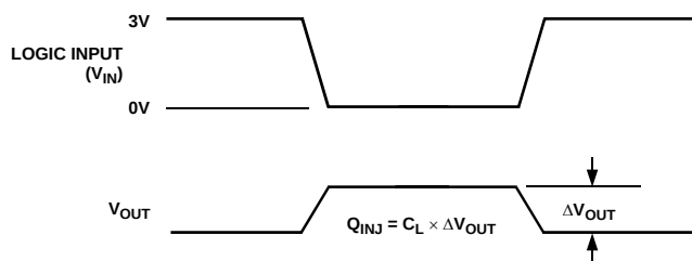
Figure 28. Charge Injection
