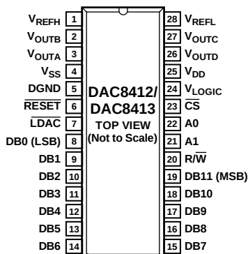
Figure 7. PDIP/CERDIP
