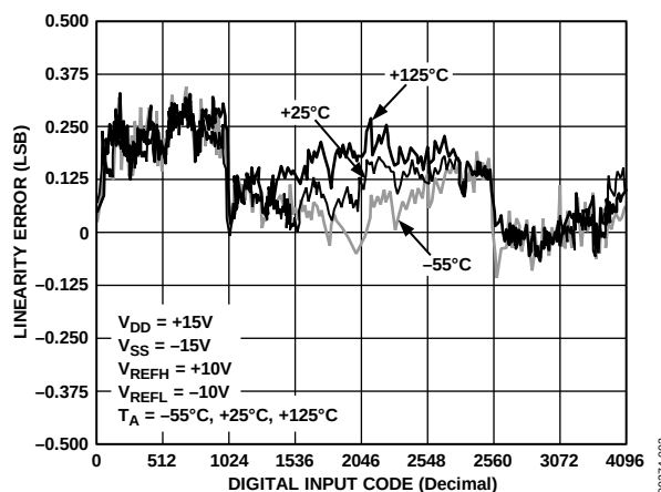
Figure 2. INL vs. Code Over Temperature
