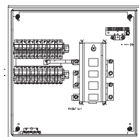
Integral Disconnect on BCBD Series 4 to 24 Circuits BCBD245-24-00B Pictured
