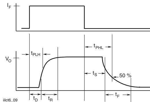
Fig. 9 - Switching Timing
