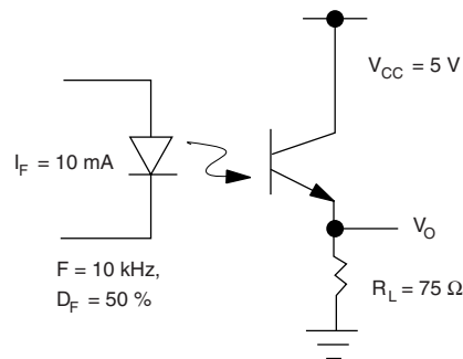
Fig. 10 - Switching Schematic
