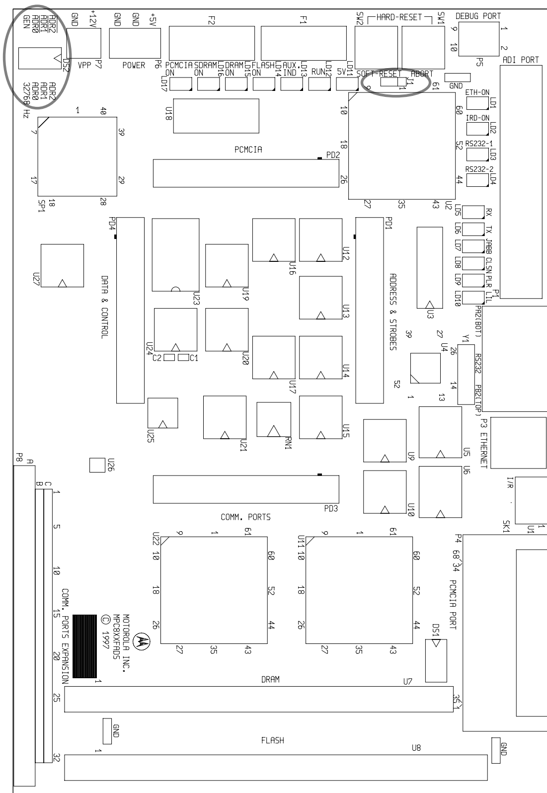
FIGURE 2-1 MPC8XXFADS Top Side Part Location diagram
