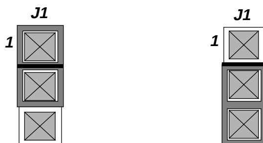
FIGURE 2-3 Power-On Reset Source Selection
