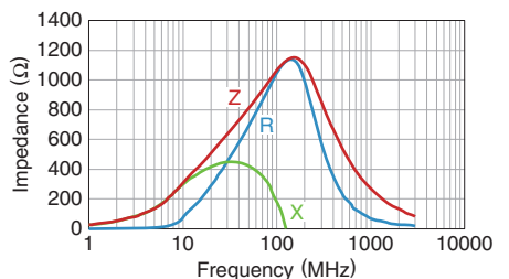
KMZ1608YHR301BTD25
