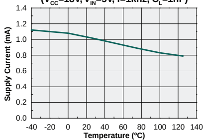
Dynamic Supply Current vs. Temperature ( V_{CC}=18V, V_{IN}=5V, f=1kHz, C_L=1nF )
