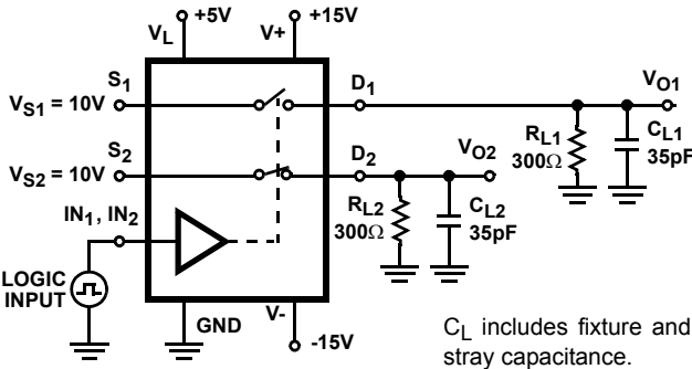
FIGURE 2B. TEST CIRCUITS
