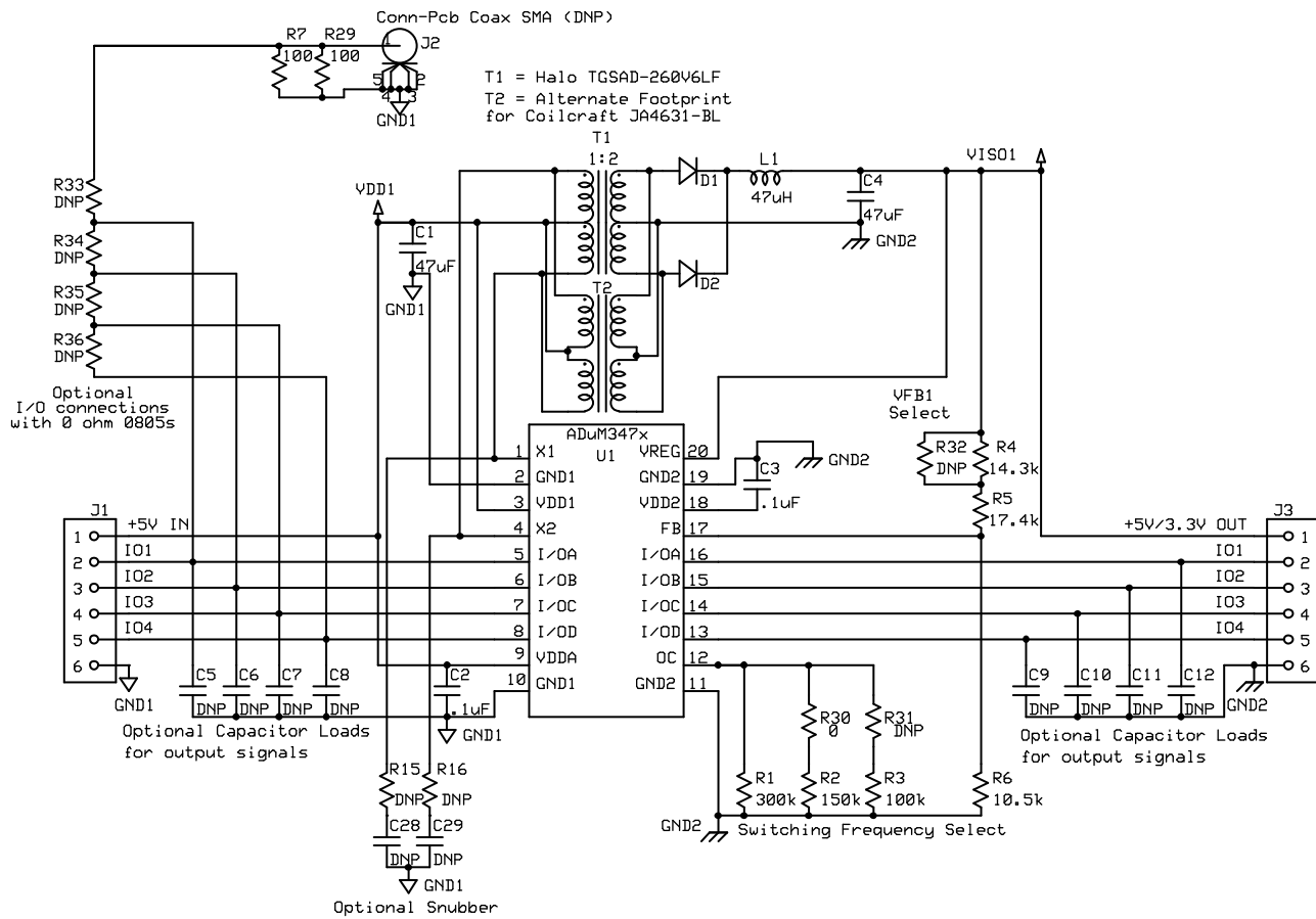
Figure 9. Single Supply Schematic
