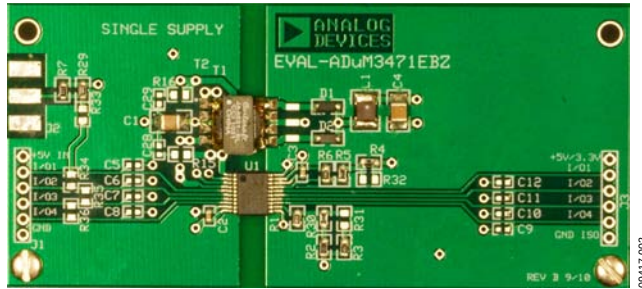
Figure 2. Single Supply
