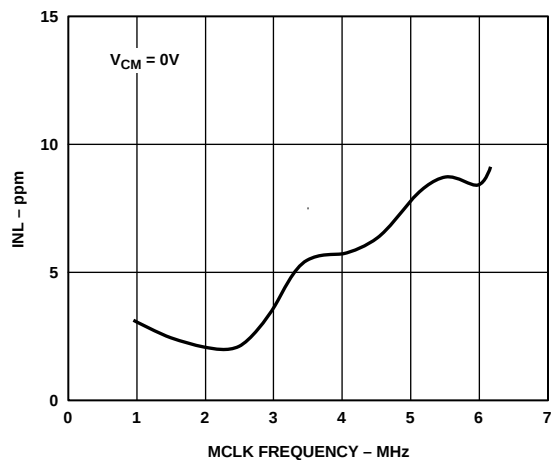
Figure 7. Typical INL vs. MCLK Frequency, \pm 10 V Differential Signal, AIN Common-Mode Voltage = 0 V, \text{BIAS}(+) = \text{BIAS}(-) = 2.5 V
