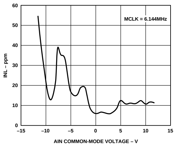
Figure 9. Typical INL vs. AIN Common-Mode Voltage, \pm 10 V Differential Signal, \text{MCLK} = 6.144 MHz, \text{BIAS}(+) = \text{BIAS}(-) = 2.5 V
