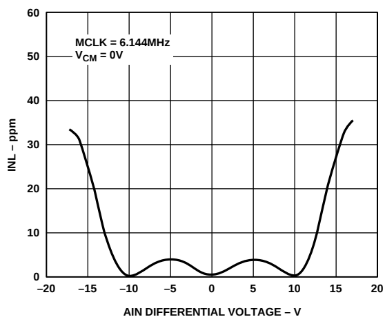
Figure 8. Typical INL vs. AIN Differential Voltage, AIN Common-Mode Voltage = 0 V, \text{MCLK} = 6.144 MHz, \text{BIAS}(+) = \text{BIAS}(-) = 2.5 V
