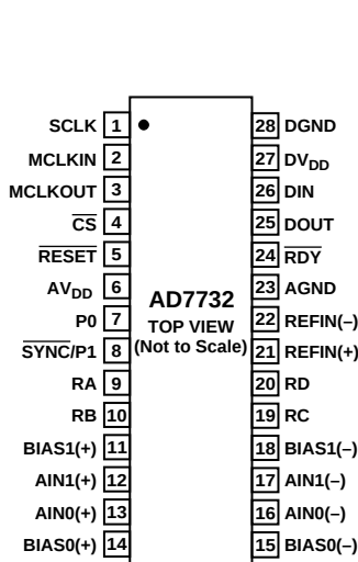
Figure 11. 28-Lead TSSOP
