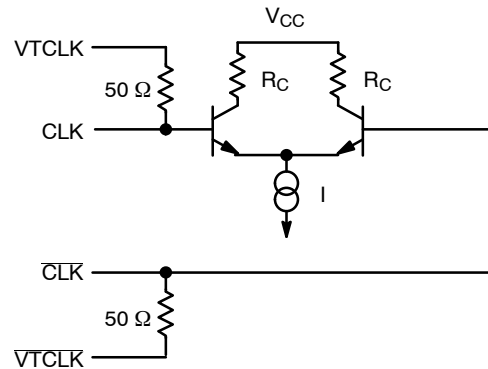
Figure 4. Input Structure
