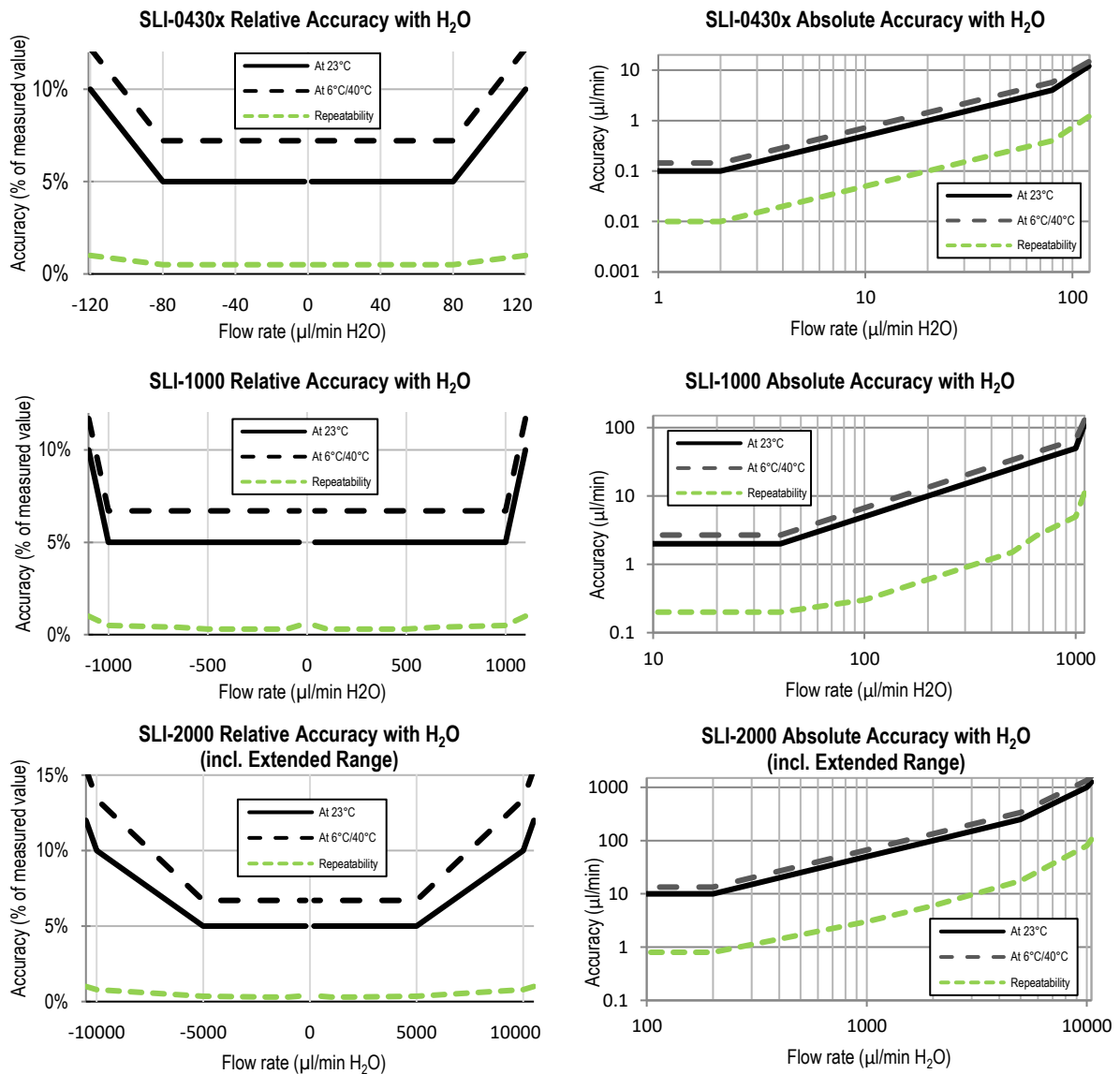
Figure 1: Flow meter accuracy and repeatability across the flow range. Relative error in % of measured value (left column) and absolute error in μl/min (right column) for H 2 O
