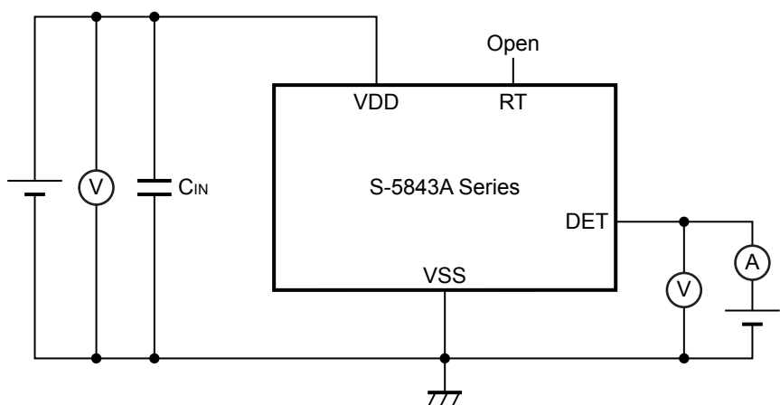
Figure 6 Test Circuit 2
