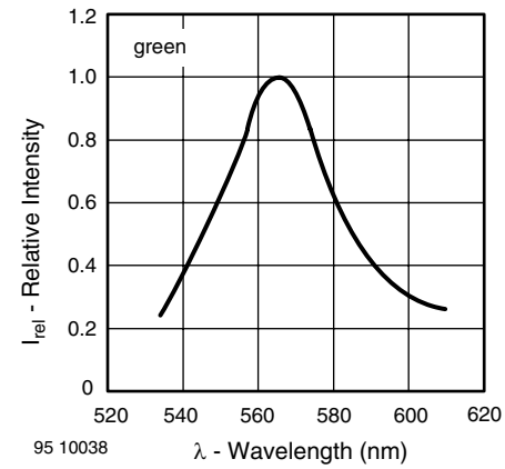
Fig. 17 - Relative Intensity vs. Wavelength
