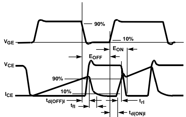
FIGURE 18. SWITCHING TEST WAVEFORM
