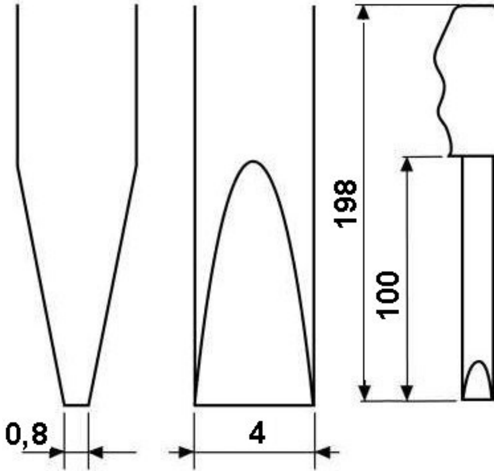
Dimensioned drawing
