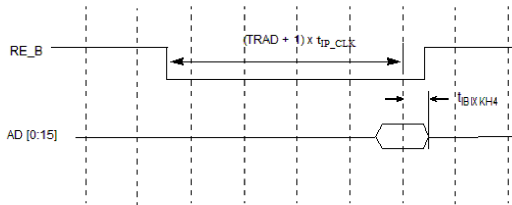
Figure 67. t_{IB|XKH4} timings
