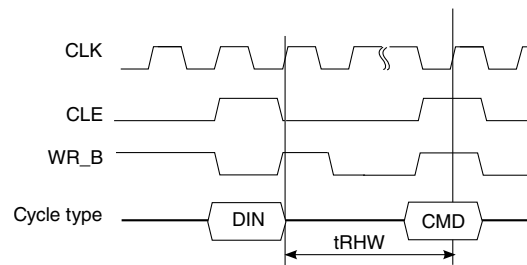
Figure 74. t_{RHW} timings
