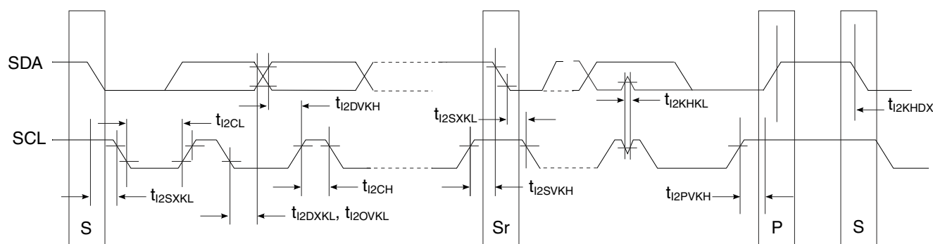
Figure 46. I²C bus AC timing diagram
