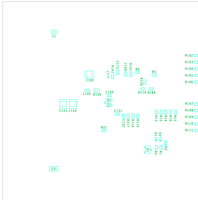
FIGURE 11. ASSEMBLY BOTTOM
