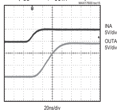
LOGIC INPUT VOLTAGE vs. OUTPUT VOLTAGE (MAX17601) (V DD = +14V, C OUTA = 10nF)
