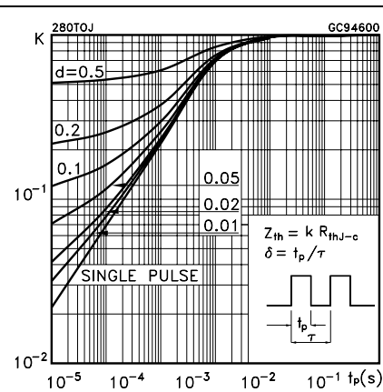
Figure 2. Thermal impedance for TO-220/ D 2 PAK/ I 2 PAK
