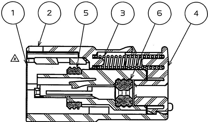
SECT. A-A
