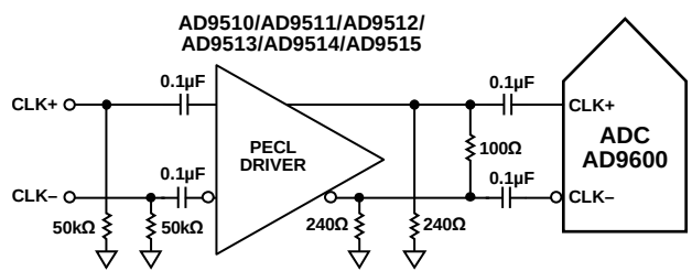
Figure 58. Differential PECL Sample Clock (up to 150 MSPS)
