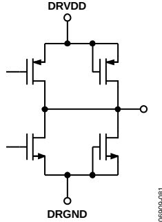
Figure 10. Digital Output
