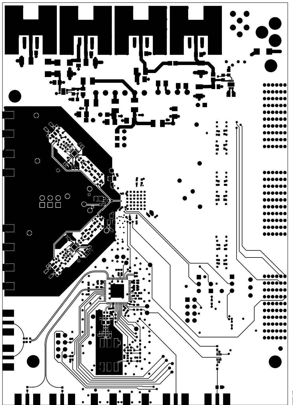
Figure 89. Evaluation Board Layout, Secondary Side (Mirrored Image)
