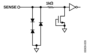
Figure 13. Equivalent SENSE Circuit
