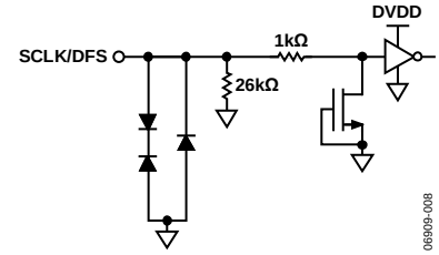
Figure 12. Equivalent SCLK/DFS Input Circuit
