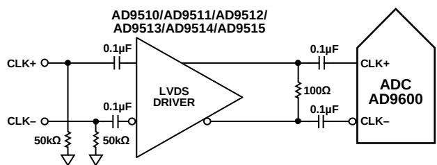
Figure 59. Differential LVDS Sample Clock (up to 150 MSPS)
