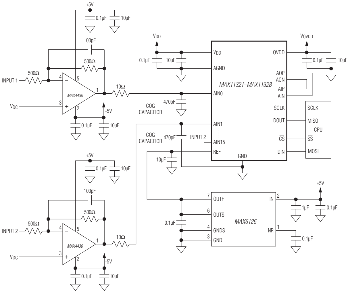
Figure 13. Typical Application Circuit
