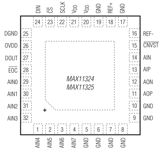
TQFN 8 CHANNEL
