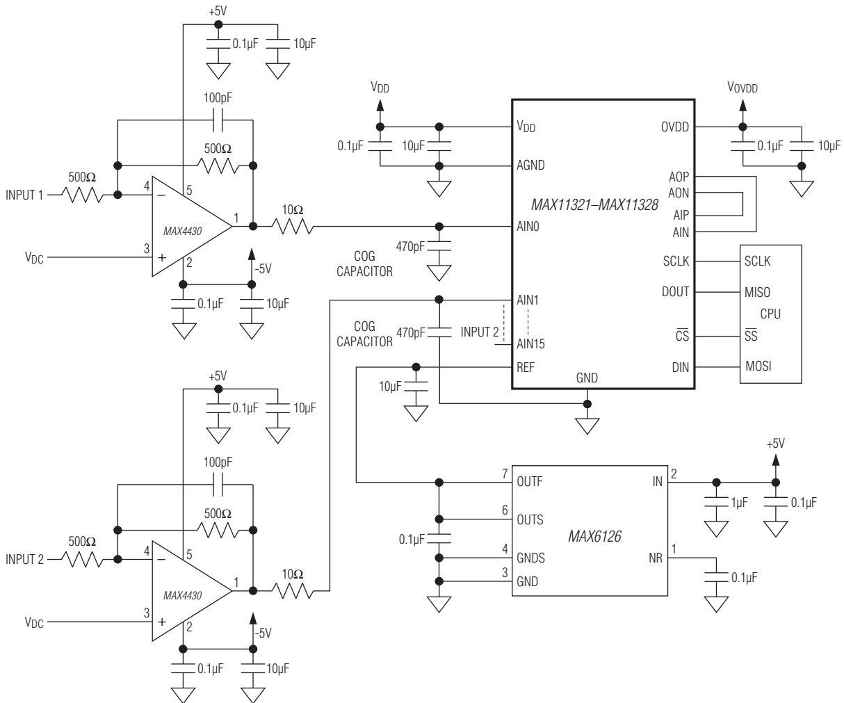
Figure 13. Typical Application Circuit
