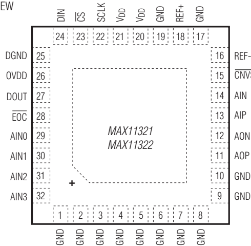
TQFN 4 CHANNEL
