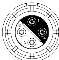
SOCKET CONTACT MATING FACE
