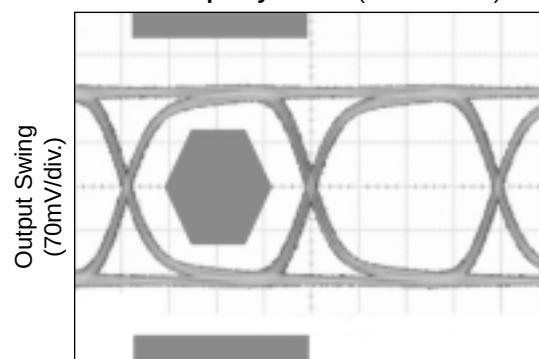
3.2Gbps Eye Mask ( 2^{23}-1 PRBS)
