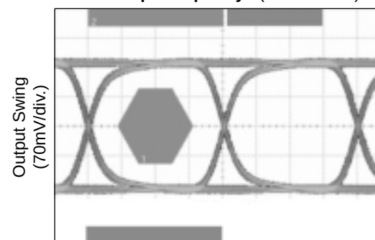
2.5Gbps Output Eye ( 2^{23}-1 PRBS)
