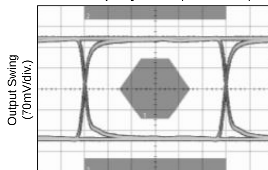
622Mbps Eye Mask ( 2^{23}-1 PRBS)
