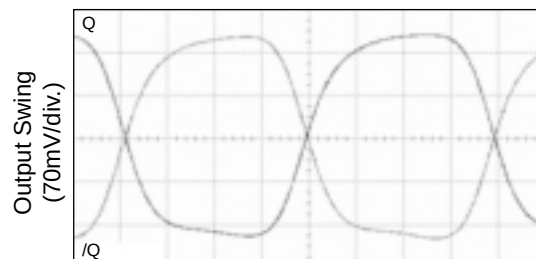
1.6GHz Output
