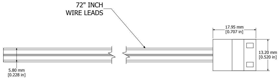
BOTTOM VIEW
