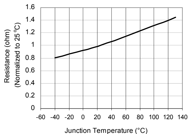
Figure 5. R ON vs. Temperature
