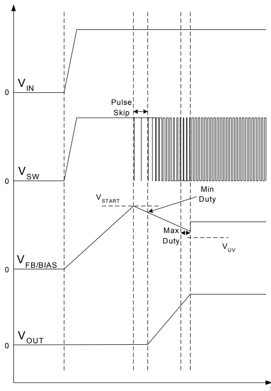
Figure 1. Power-up waveforms
