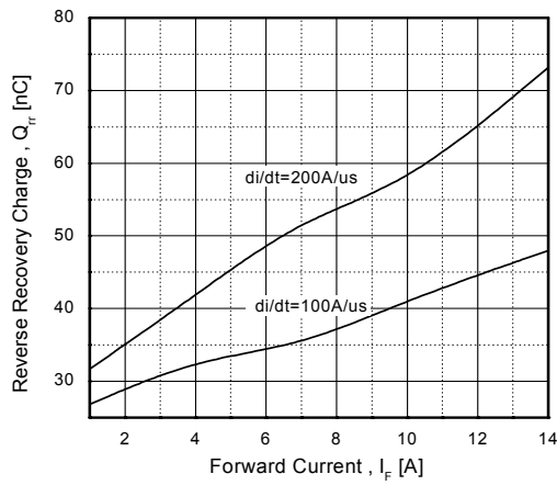
Figure 19. Stored Charge
