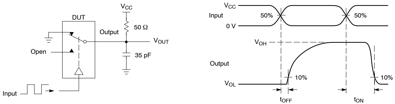
Figure 2. t_{ON}/t_{OFF}
