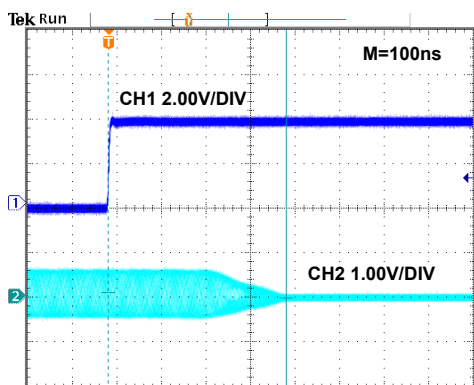
FIGURE 17. DISABLED RESPONSE
