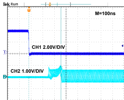
FIGURE 18. ENABLED RESPONSE
