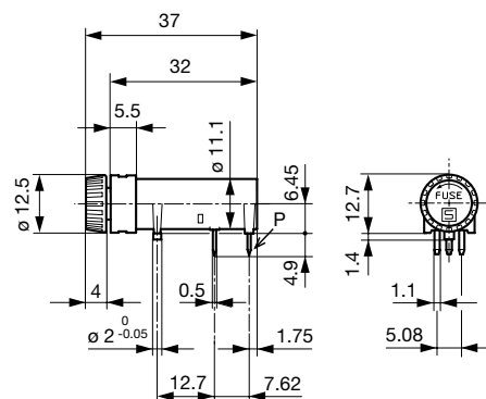
Variant Fingerrip 3101.0055 / Connector tinned
