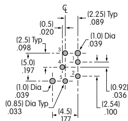
PCB Footprint
