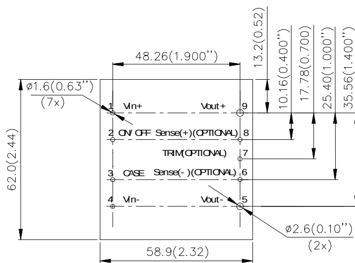
RECOMMENDED PWB LAYOUT
