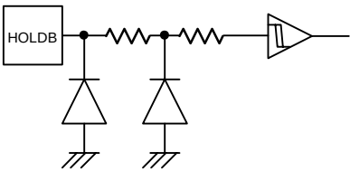
Figure 58. HOLDB input equivalent circuit
