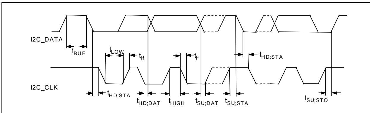
FIGURE 43-11: I2C/SMBUS TIMING
